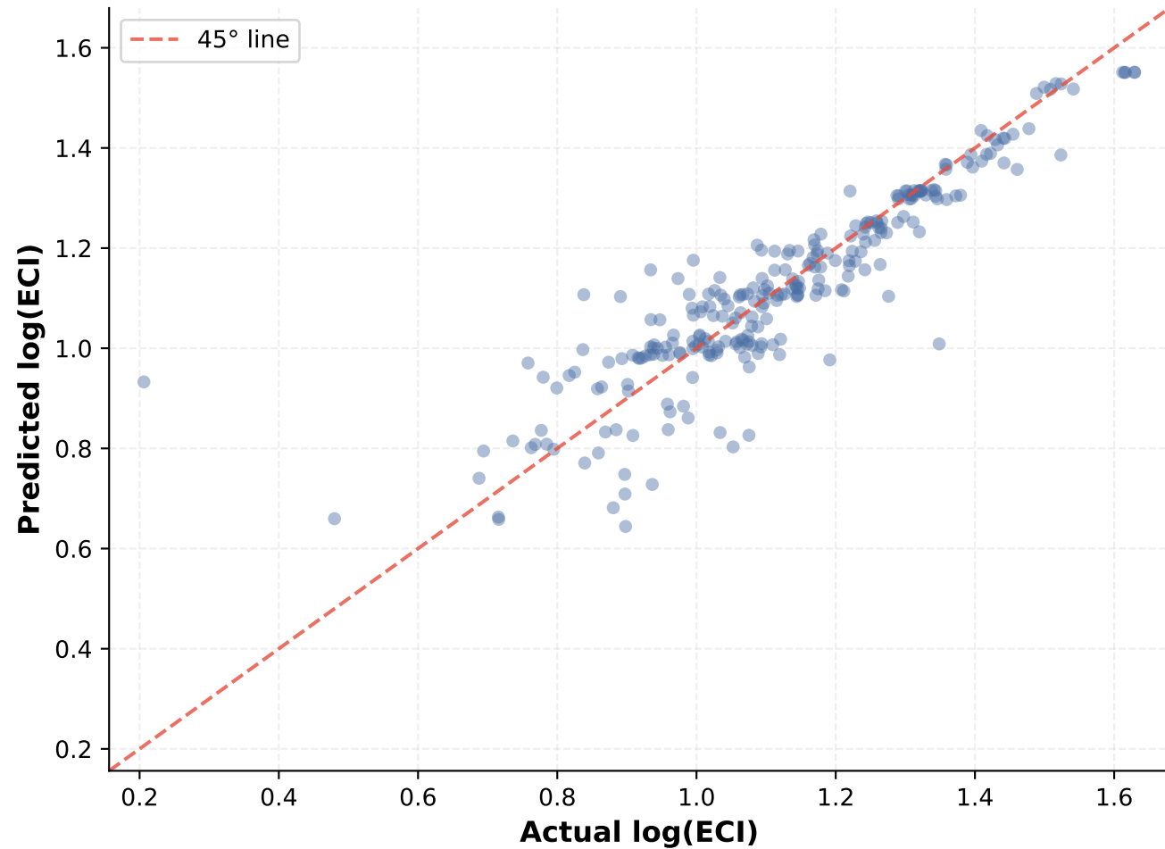
Random Forest — \log(\text{ECI}) Test R^2=0.809 | RMSE=0.0905
